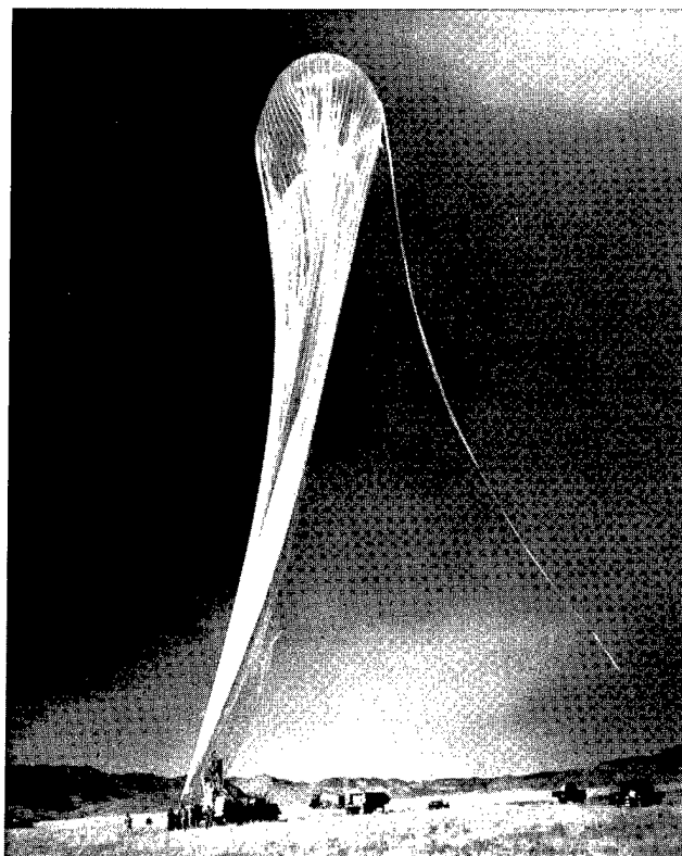
Fig. 81. Scene typical of a mid- to late 1950s off-range high altitude balloon launch. (U.S. Air Force photo)
